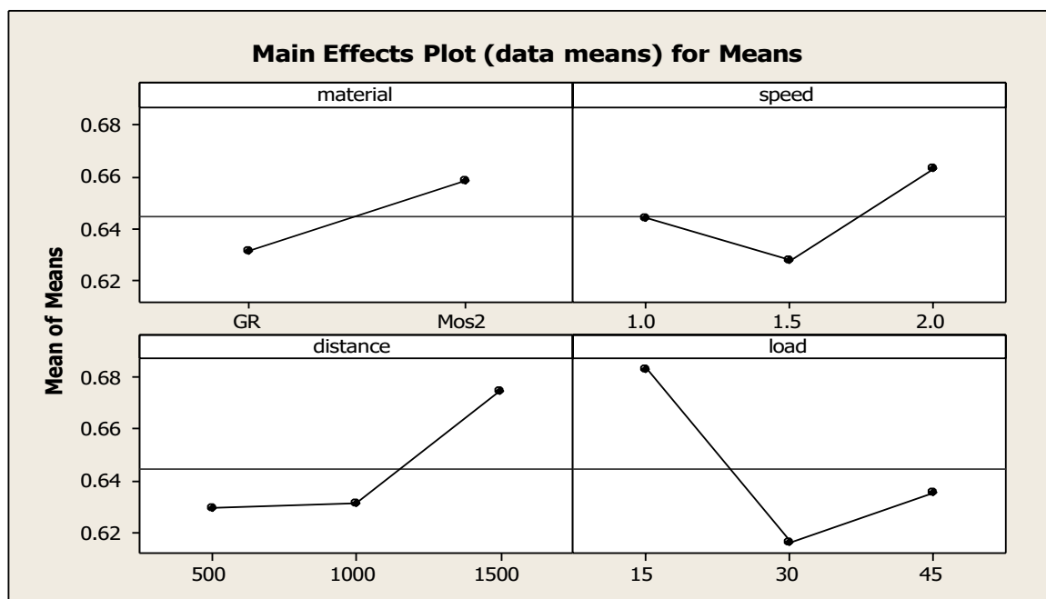
Fig.3 Response Graphs of 356/ 6% B4C/ 2% Gr, 2% MoS 2 Composites
