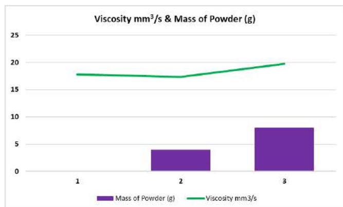
FIGURE 7. Viscosity and Mass of Walnut Shell Particles
