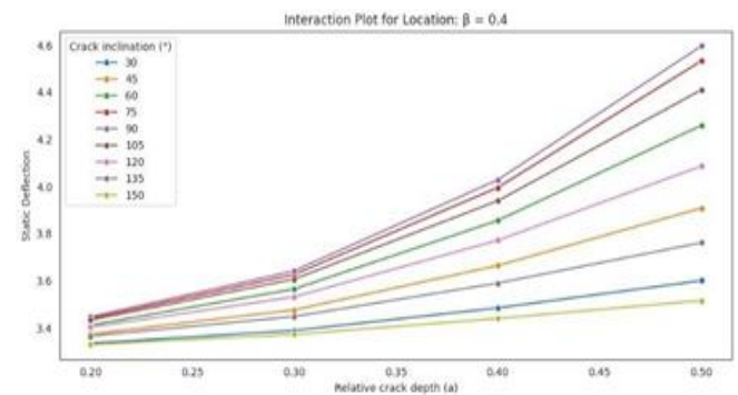
Figure 20 Interaction plots for Location: \beta = 0.4 in Timoshenko Beam
