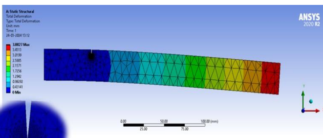
Figure 7 Static Deflection Obtained for Timoshenko Beam with Crack
