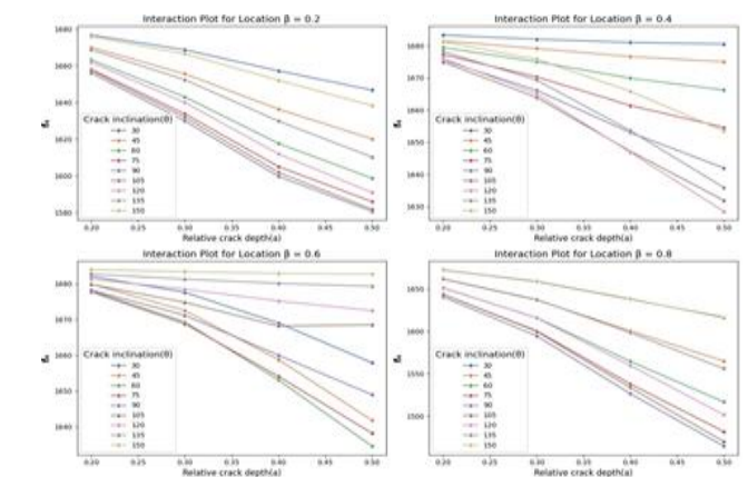
Figure 35 Interaction plot for f4 at all Locations ( \beta ) in Euler Bernoulli Beam
