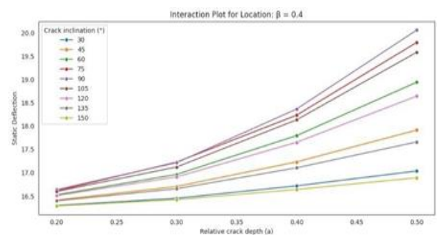
Figure 21 Interaction plots for Location: \beta = 0.4 in Euler Bernoulli Beam
