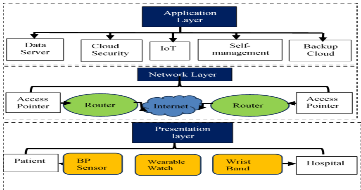
Figure 2 Multi-Layer Model
