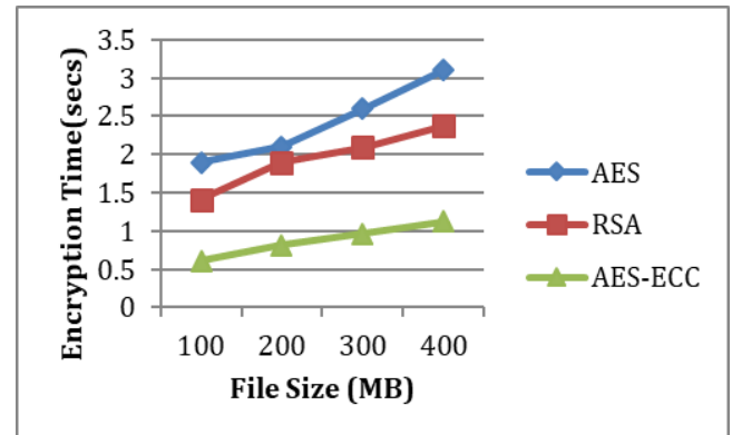
Figure 6 Encryption Time
