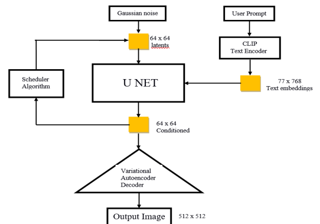
Figure 2 Algorithm
