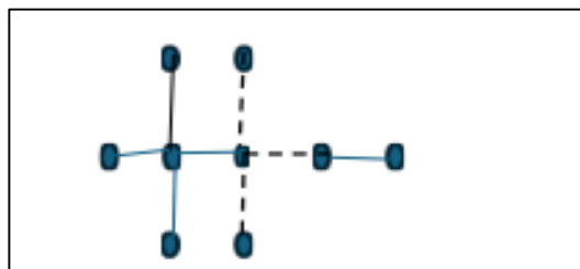
Figure 2 Ethanol
