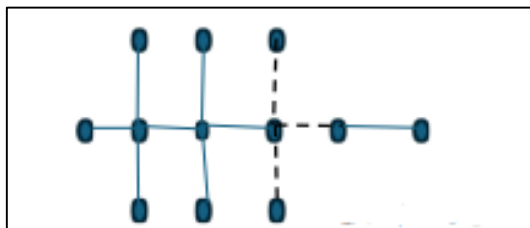
Figure 3 Propanol
