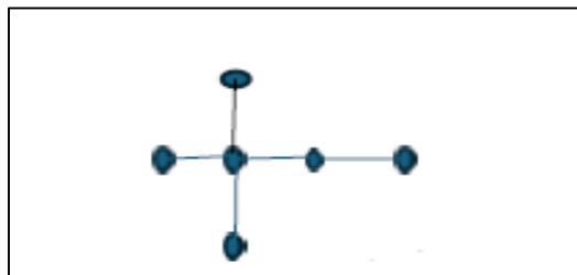
Figure 1 Methanol
