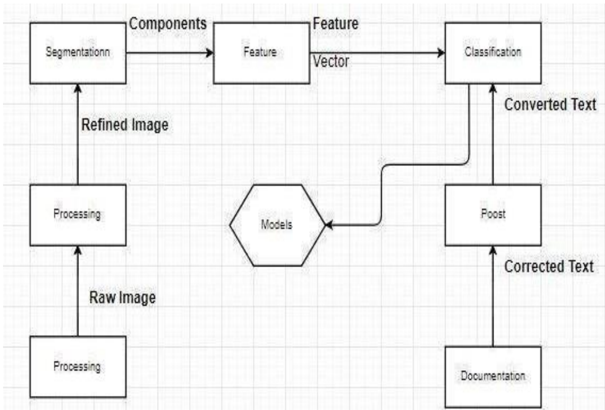
Fig 1. Image Classification
